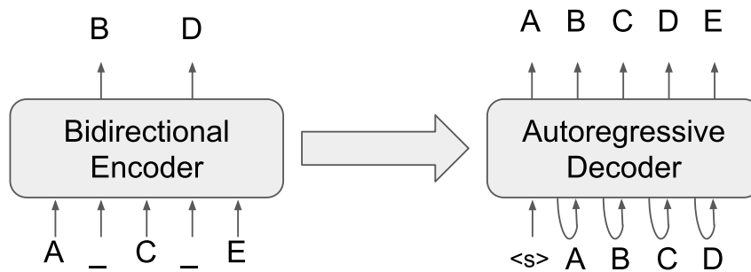
Figure 9: Scematic architecture of the Bidirectional and Auto-Regressive Transformer.
