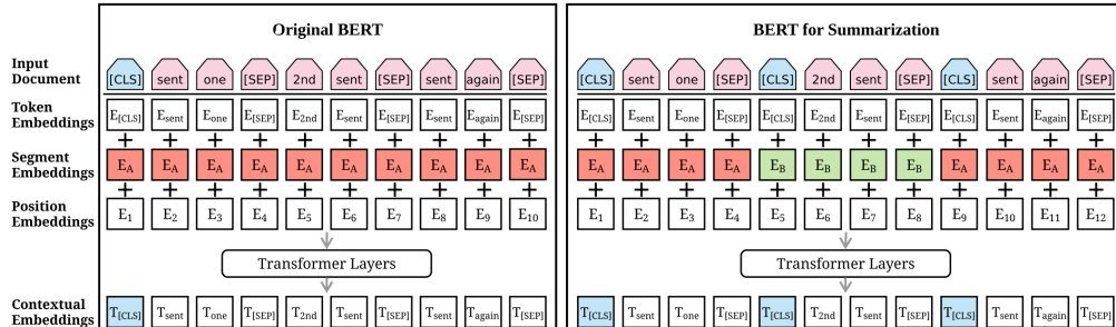
Figure 8: Overview of BERT architectures: The original BERT is displayed on the left, the for summarization adapted BERT on the right.
