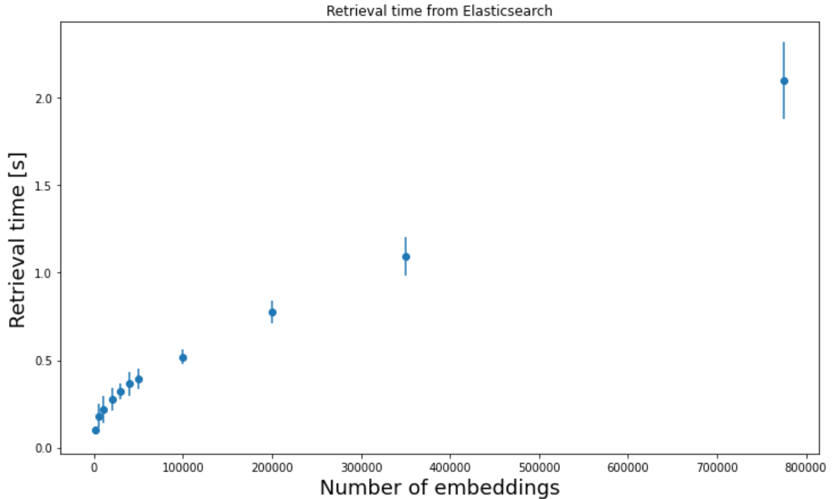
Figure 2: A plot comparing the retrieval time in seconds for a single image embedding query as the size of the index i.e. the number of embeddings increases.
