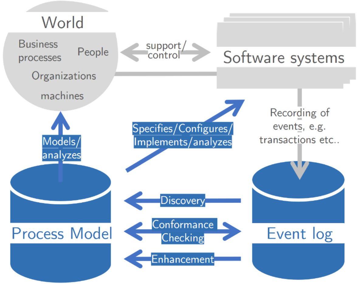
Figure 1.1: An overview about Process Mining (Aalst 2016, p. 32).
